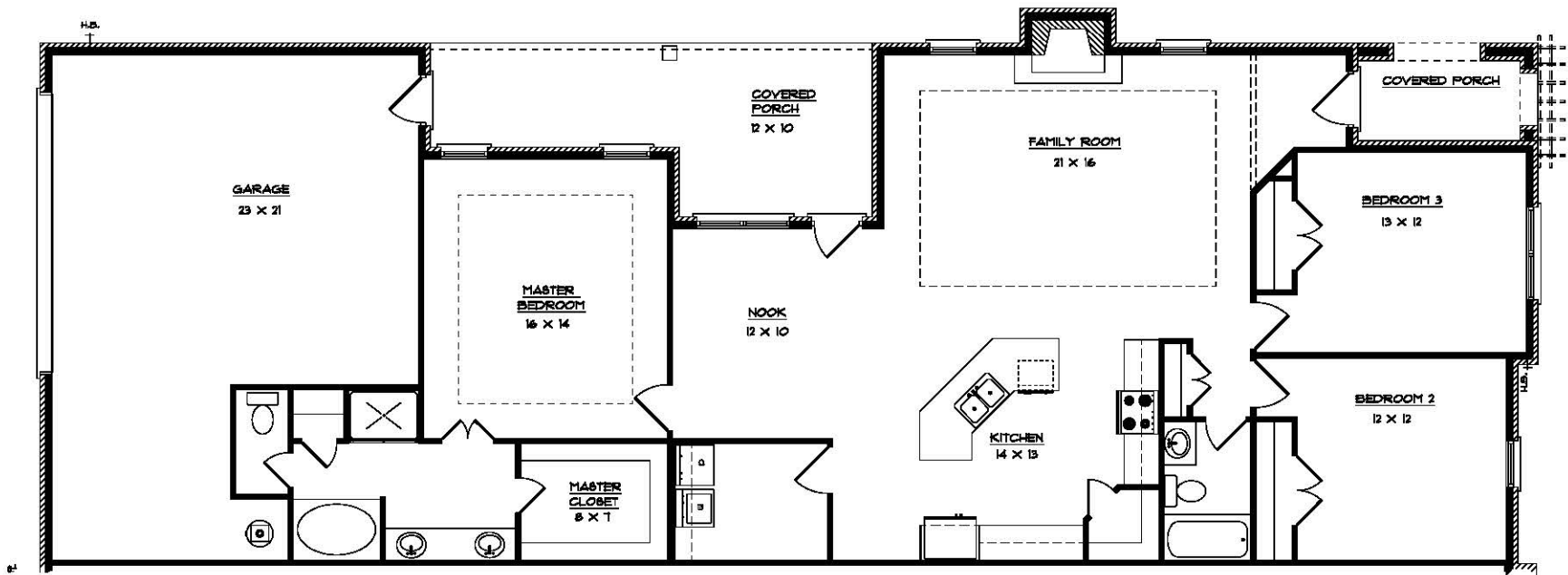
FLOOR PLAN
