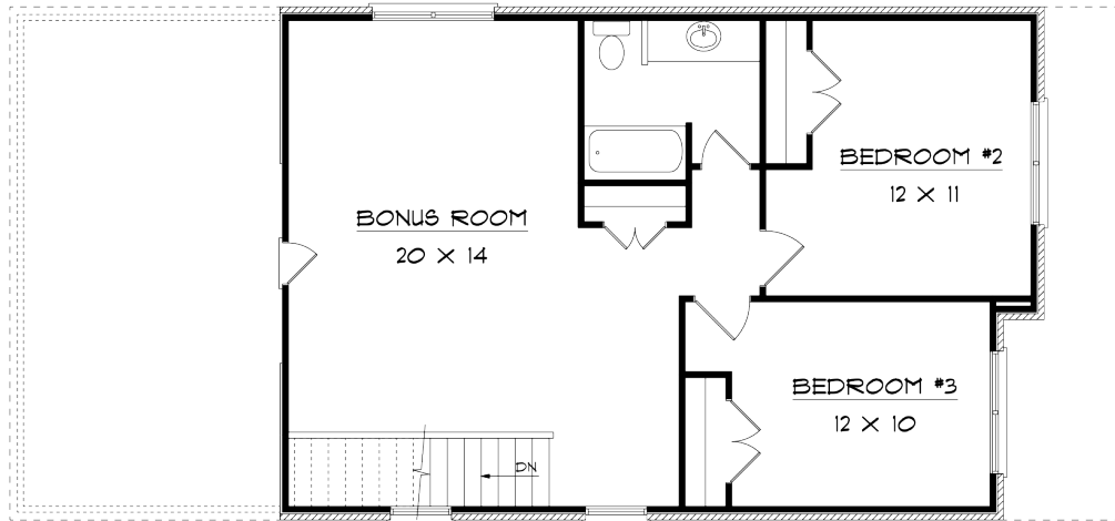
2nd Floor
