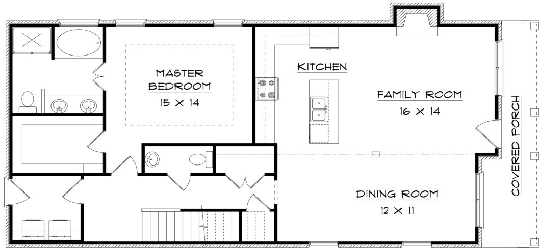
1st Floor
