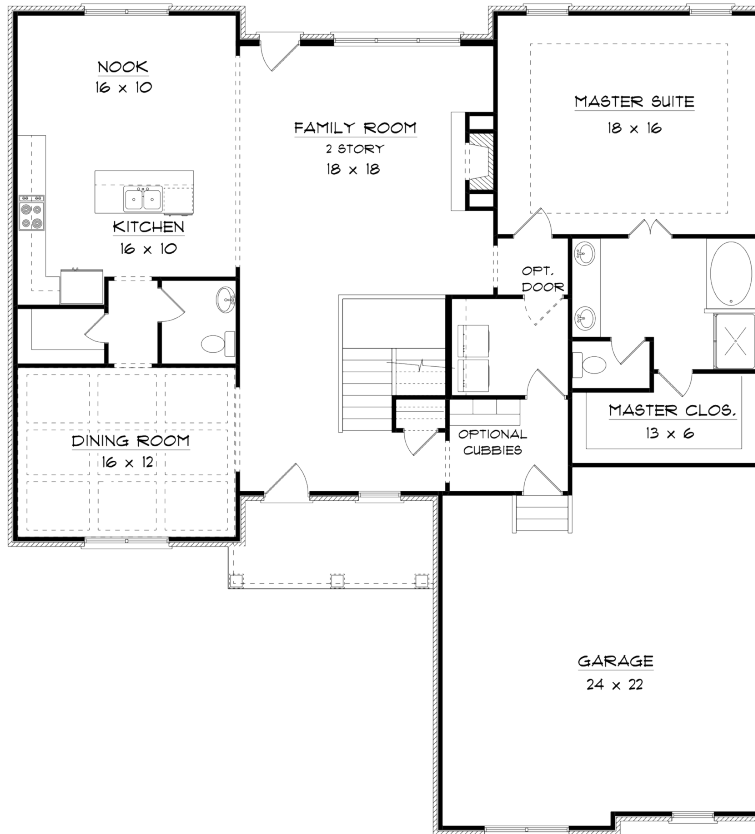
1st Floor
