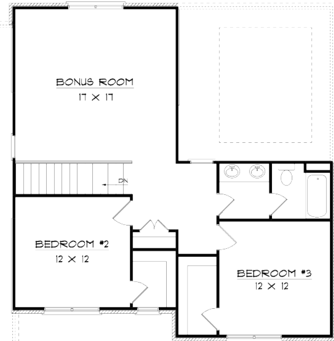
2nd Floor
