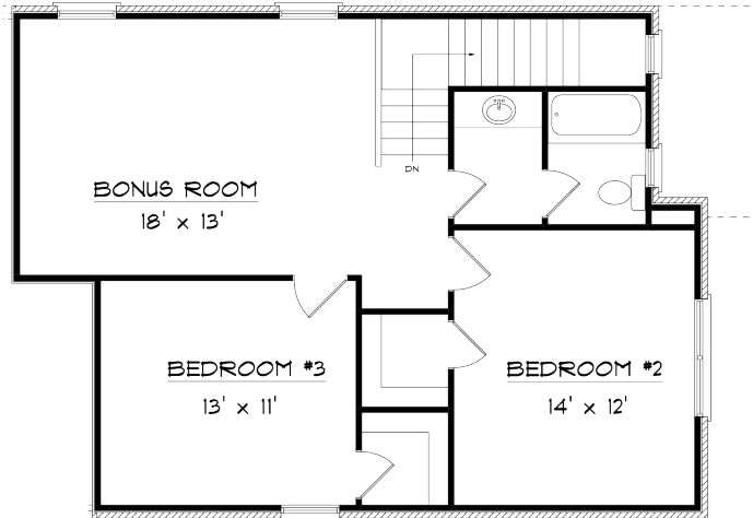
2nd Floor
