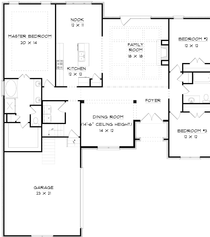
1st Floor
