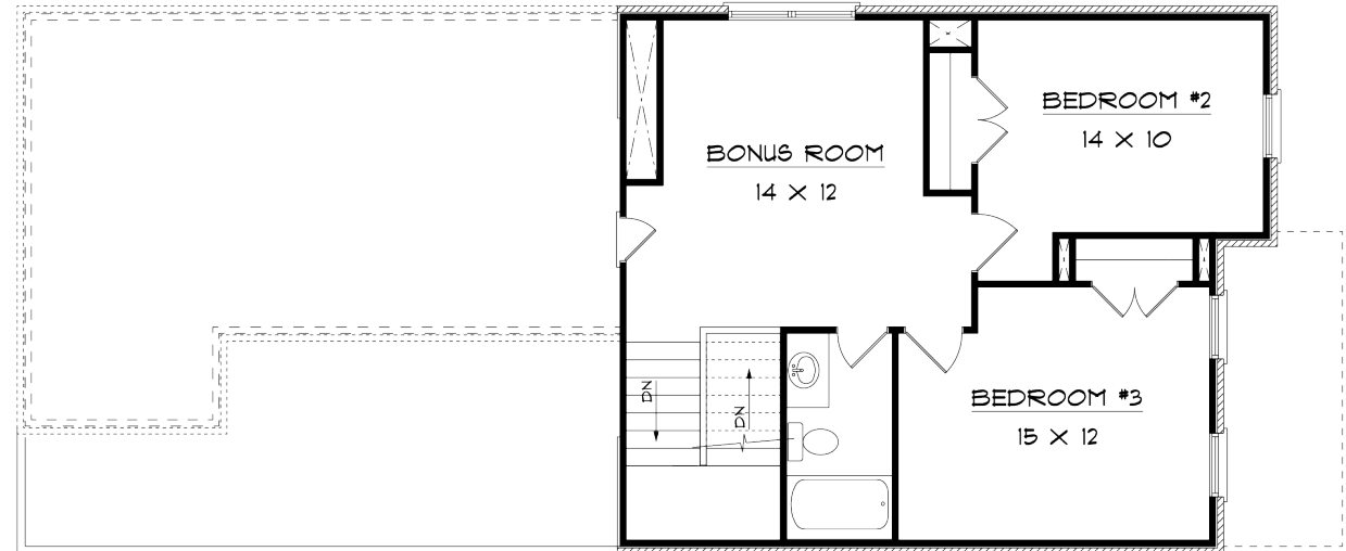
2nd Floor
