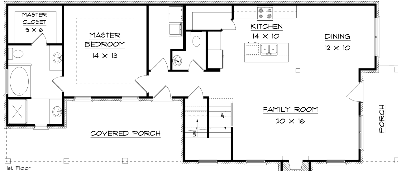
1st Floor
