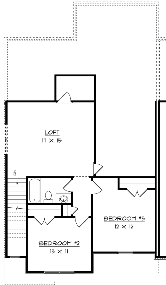
SECOND FLOOR
